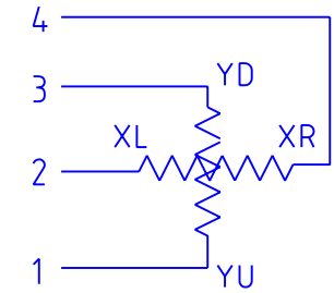
PIN ASSIGNMENT
